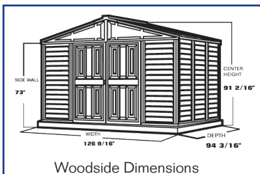
Woodside Dimensions
